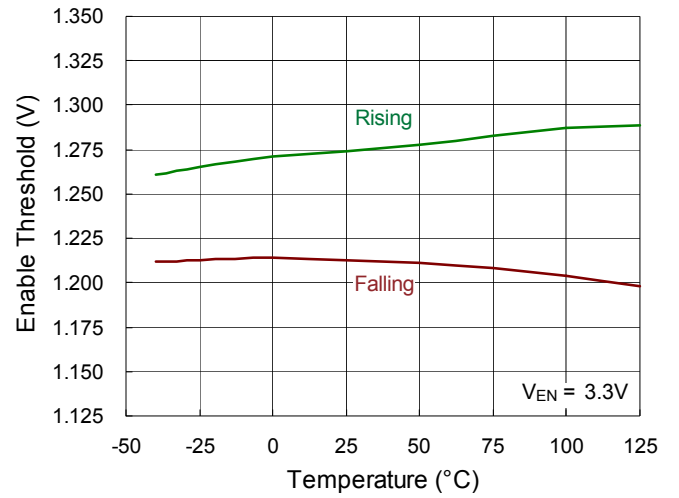
Enable Threshold vs. Temperature
