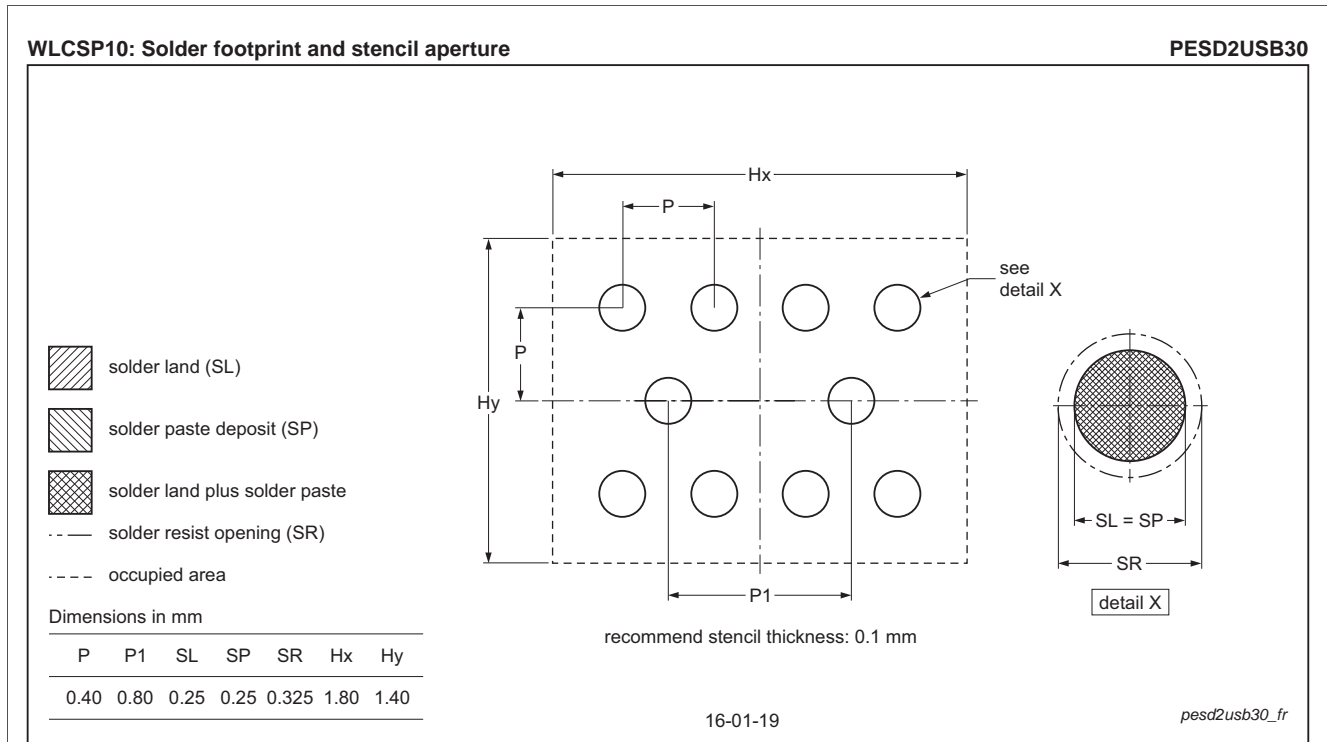
Fig 19. Soldering footprint WLCSP10 (PESD2USB30)
