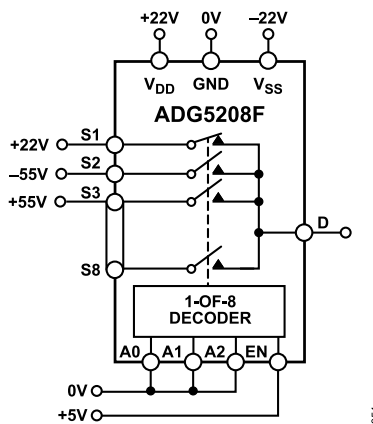
Figure 51. ADG5208F in an Overvoltage Condition
