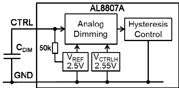
Figure 36 Soft Start
