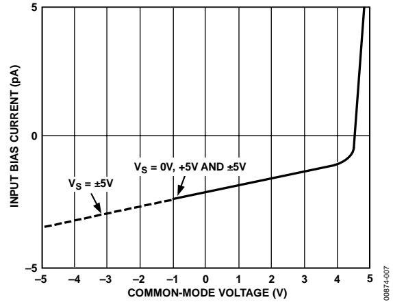
Figure 7. Input Bias Current vs. Common-Mode Voltage; VS = 5 V, 0 V, and VS = ±5 V
