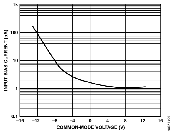
Figure 8. Input Bias Current vs. Common-Mode Voltage; VS = ±15 V
