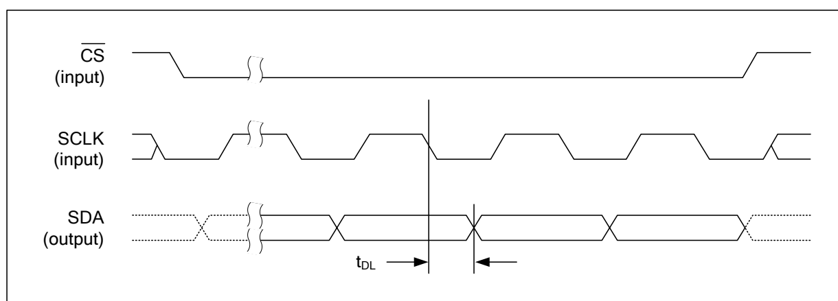
Figure 9 Control Interface Timing - 3-wire (SPI) Control Mode (Read Cycle)
