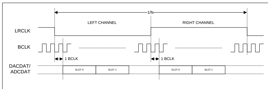
Figure 59 TDM in I²S Mode
