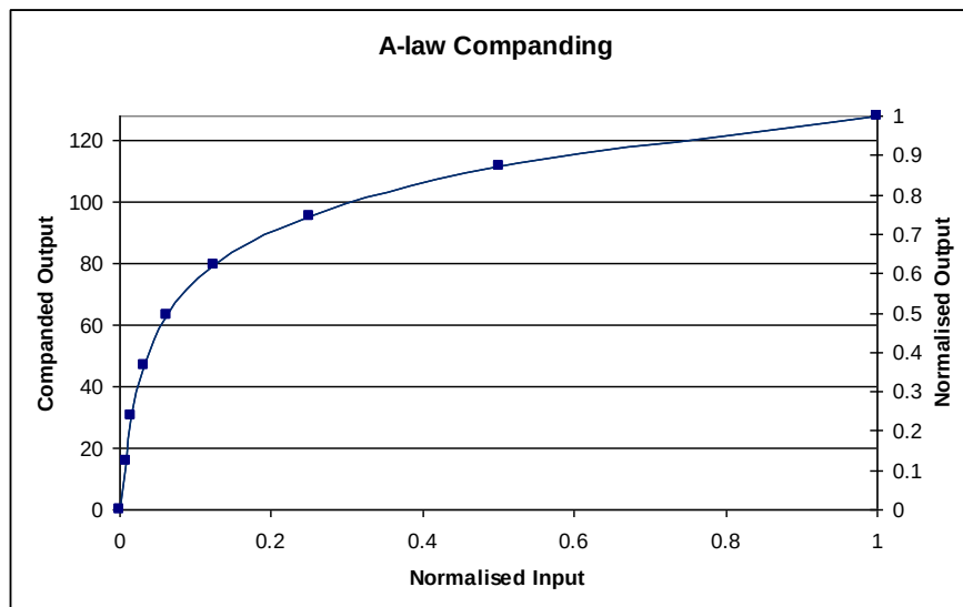
Figure 64 A-Law Companding
