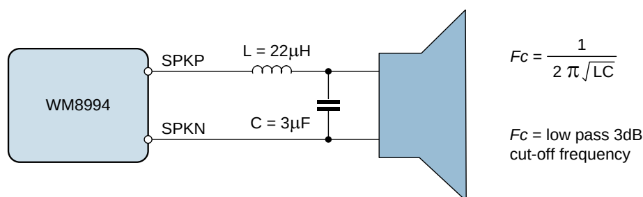
Figure 92 Class D Output Filter Components
