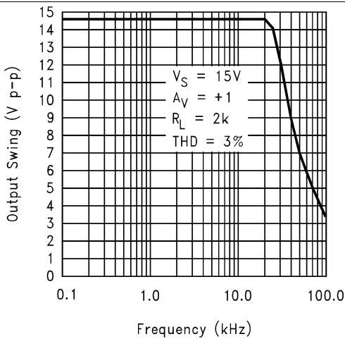
Figure 37. Maximum Output Swing vs Frequency
