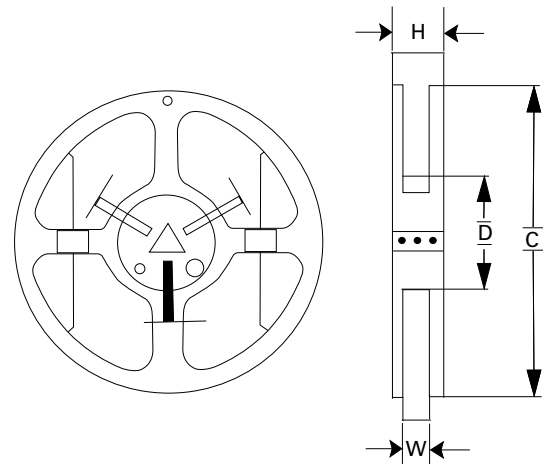
Reel Specifications
