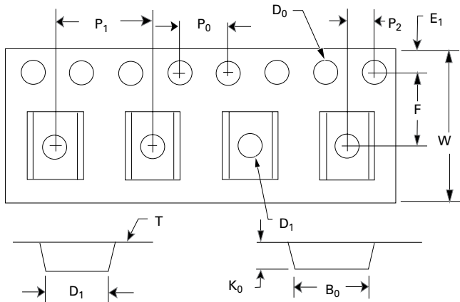
Tape Specifications
