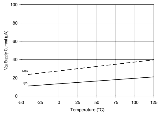
Figure 19A. V DS Supply Current vs. Temperature
