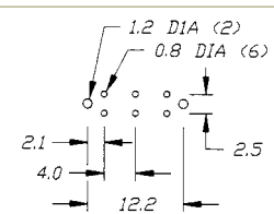
P.C. MOUNTING
