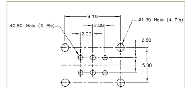
P.C. MOUNTING
