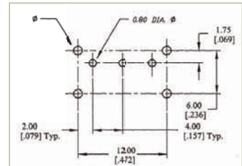
P.C. MOUNTING
