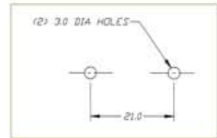
PANEL MOUNT
