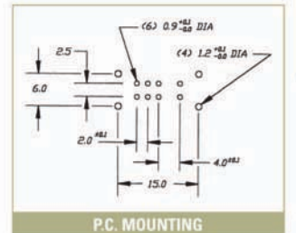
P.C. MOUNTING
