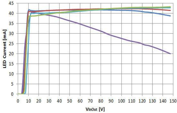
Figure 10. LED Current (-40°C to +105°C) vs. V_{IN\_OUT}
