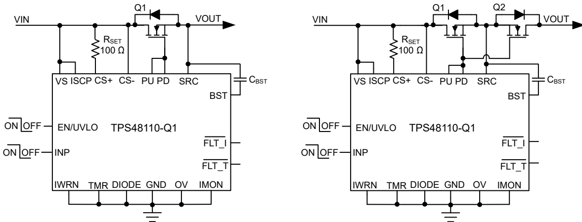
Figure 8-16. Connection Diagram of TPS4811-Q1 for Simple Gate Driver Design
