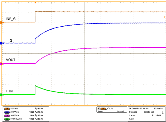
Figure 9-15. Pre-charge Profile of the Output Capacitance ( V_{IN} = 48\text{ V} , C_{OUT} = 440\ \mu\text{F} , No Load)
