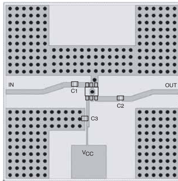
Figure 2. Evaluation Board
